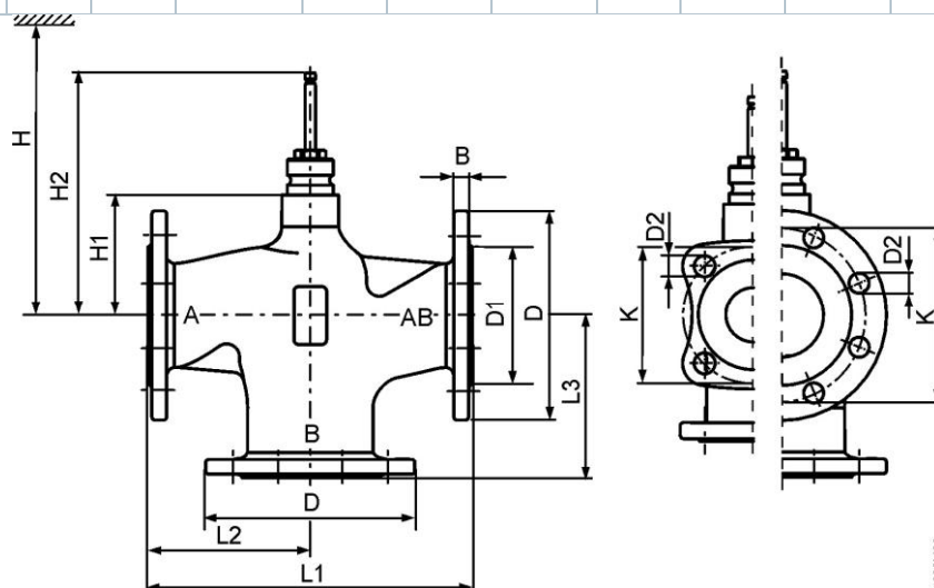
VXF42..C
