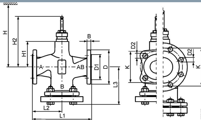
VVF42..C, VVF42..KC
